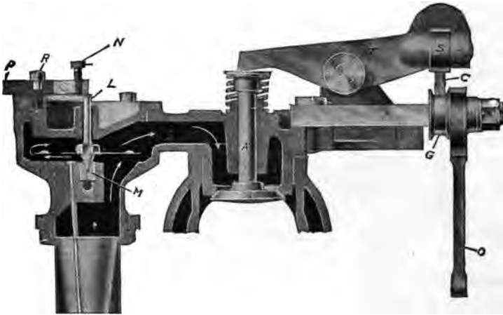
FIG. 238.—Carburetor and Intake Valve of the Cadillac One-Cylinder Engine. L is the gasoline valve; M, gasoline inlet; N, adjusting screw. A, inlet valve; T, walking-beam for opening it under positive impulse; C, end of eccentric rod, raising T by bearing on roller, S, with roller, G, as fulcrum. O is the handle by which the position of G, consequently the lift of the valve, A, may be varied as desired.
